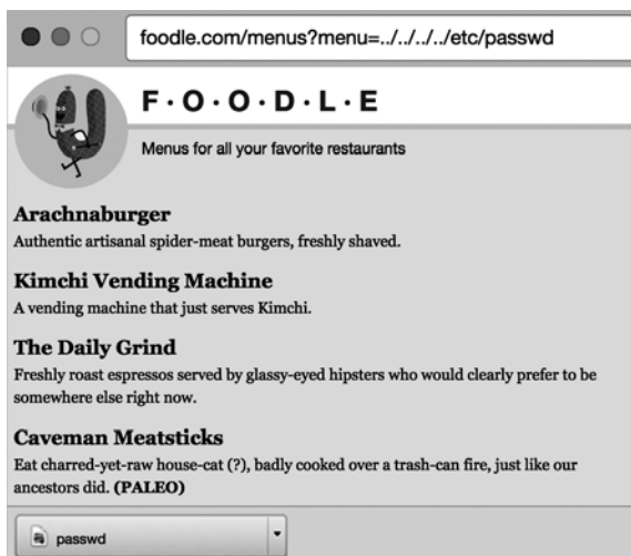
Figure 11-2: Using a directory traversal attack to access a Unix file holding account information
